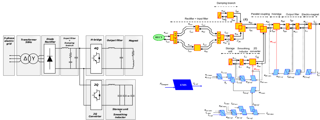
Figure 1 : POLARIS elementary block and its maximal control scheme
