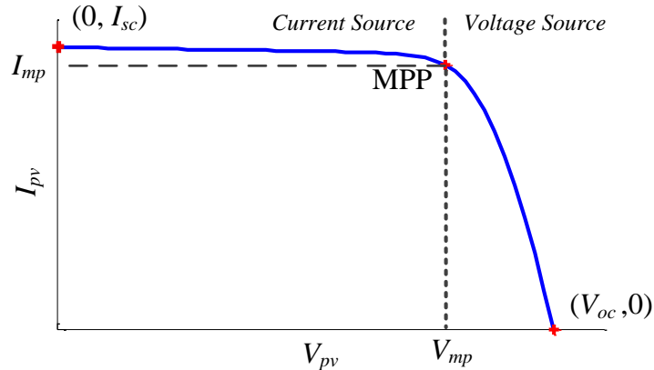
Figure AIII-2 Characteristic I-V curve of a practical photovoltaic device and the three remarkable points: short circuit (0, I_{sc}) , maximum power point (V_{mp}, I_{mp}) and open-circuit (V_{oc}, 0) .
