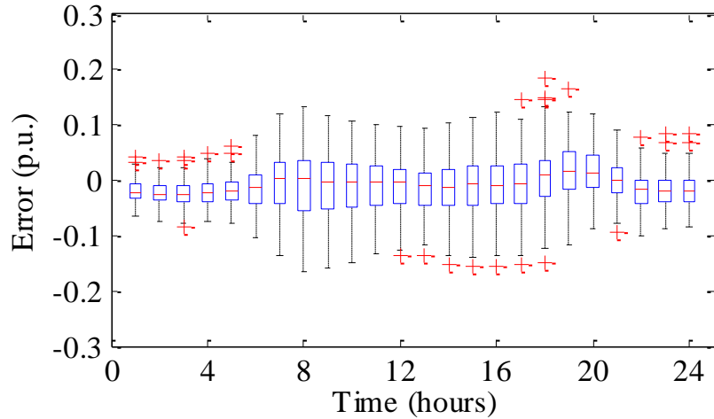
Figure II-22 Load demand prediction errors with data from the test set.
